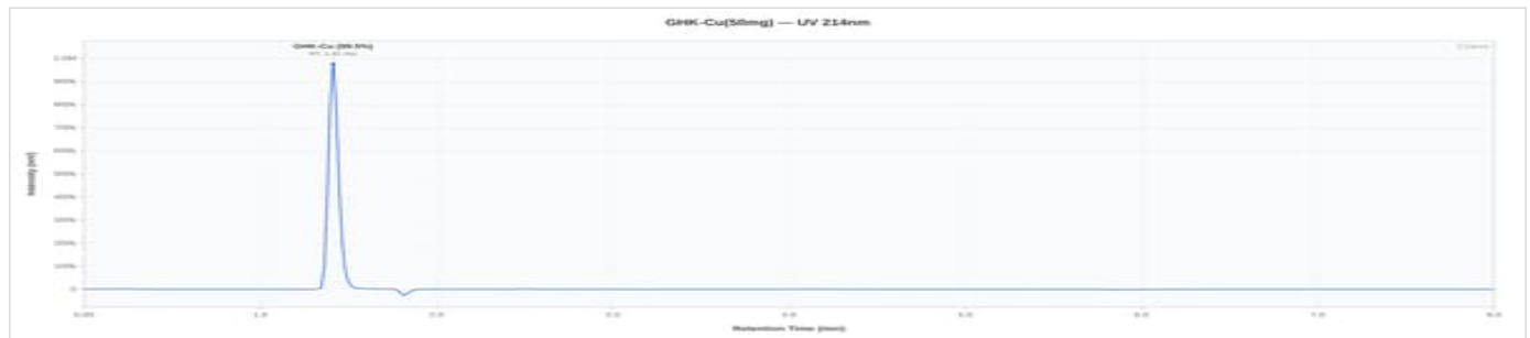
GHK-Cu 50mg - 2026-0731: UV Chromatogram
